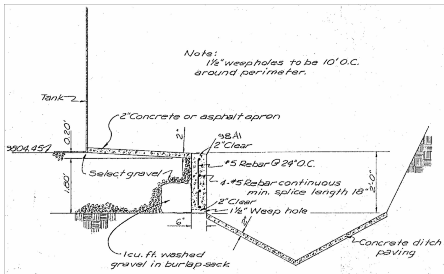
1 - EXISTING RINGWALL DETAIL NOT TO SCALE
